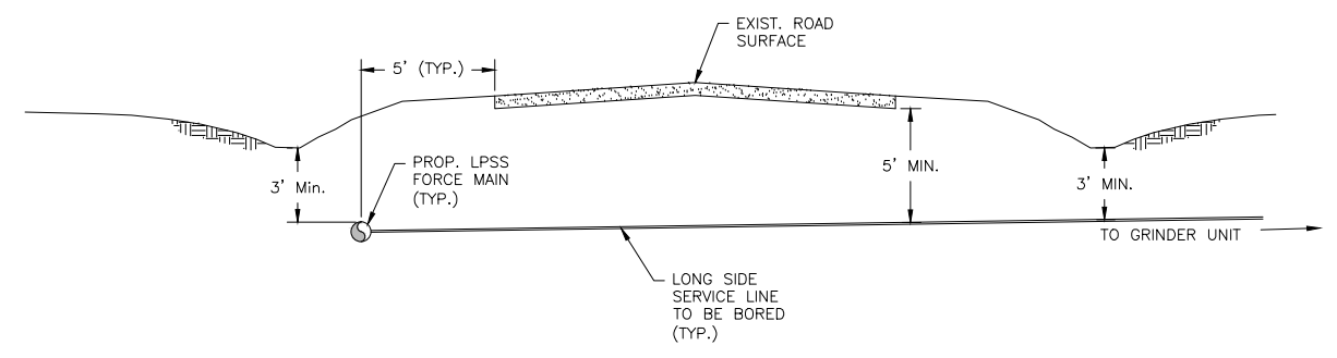
INSTALLATION DETAIL FOR LONG SIDE SERVICES CROSSING COUNTY ROADS (TYPICAL)
