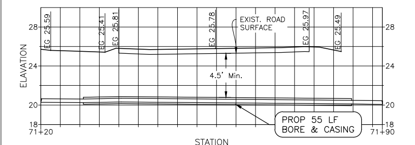
PROFILE VIEW LPSS FORCE MAIN CROSSING LAWHON & MLK INTERSECTION
