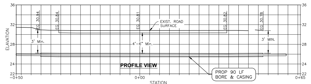
PROFILE VIEW LPSS FORCE MAIN CROSSING BOYT ROAD & LAWHON INTERSECTION
