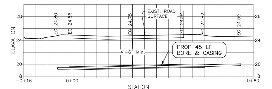
PROFILE VIEW LPSS FORCE MAIN CROSSING LAWHON & KIDD RD. INTERSECTION
