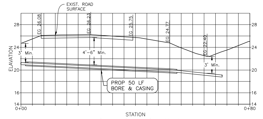
PROFILE VIEW LPSS FORCE MAIN CROSSING BOYT ROAD
