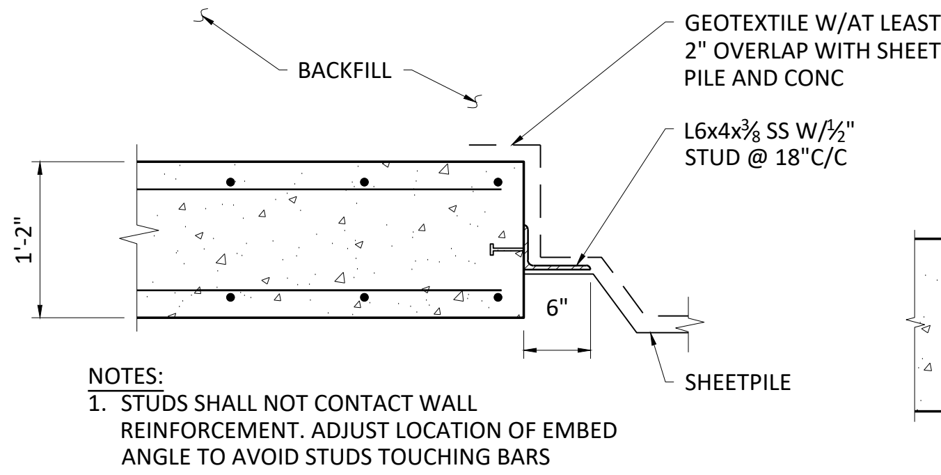
1 S-02 1"=1'-0" SHEETPILE TO WALL CONNECTION DETAIL
