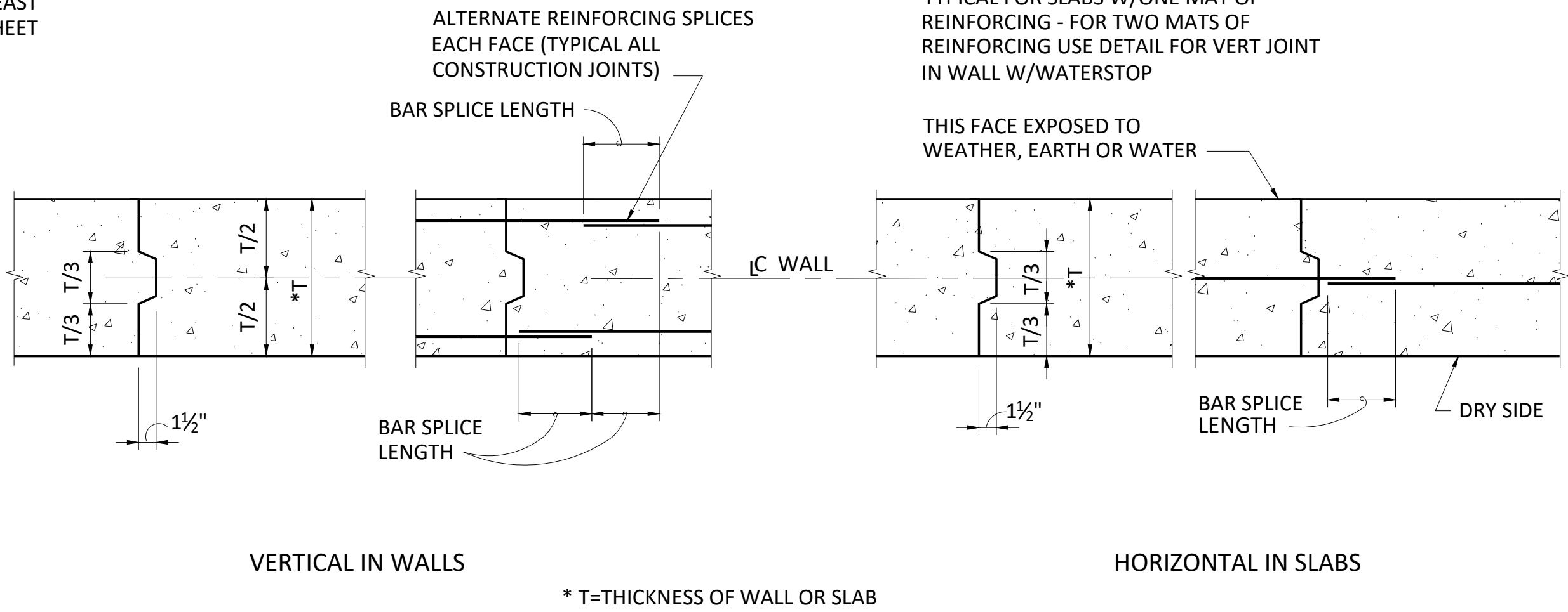
2 - NOT TO SCALE CONSTRUCTION JOINTS DETAILS
