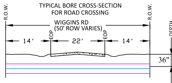
CROSS SECTION NOTES & SPECIFICATIONS 1. CONDUITS SHALL BE 3 FEET FROM ROW LINE
