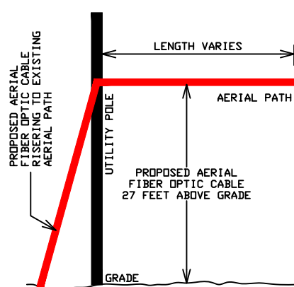
TYPICAL AERIAL PROFILE FOR EXISTING POLES & EXISTING AERIAL PATHS
