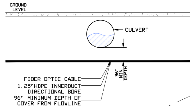
CULVERT CROSSING PROFILE S GARDEN DR
